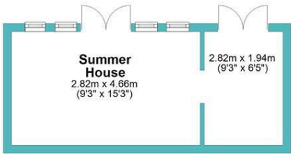
Summer House Approx. 18.9 sq. metres (203.6 sq. feet)
